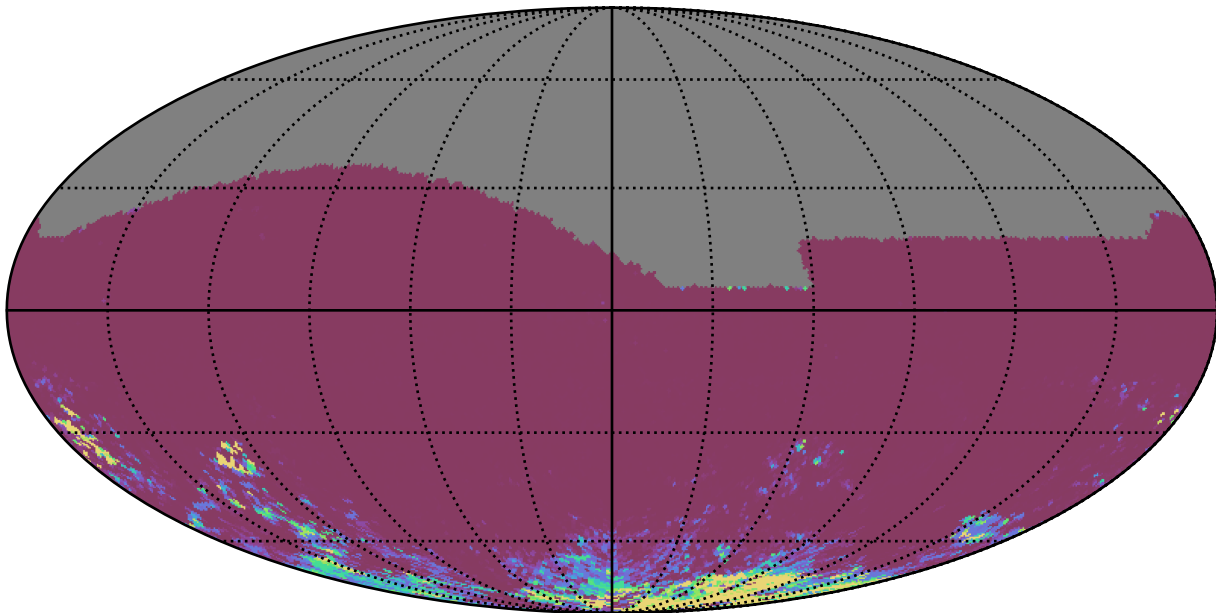
too_elab_heavy_r32_d2_griz_v3.4_10yrs All sky ri bands: 75th Percentile Intranight Timespan
