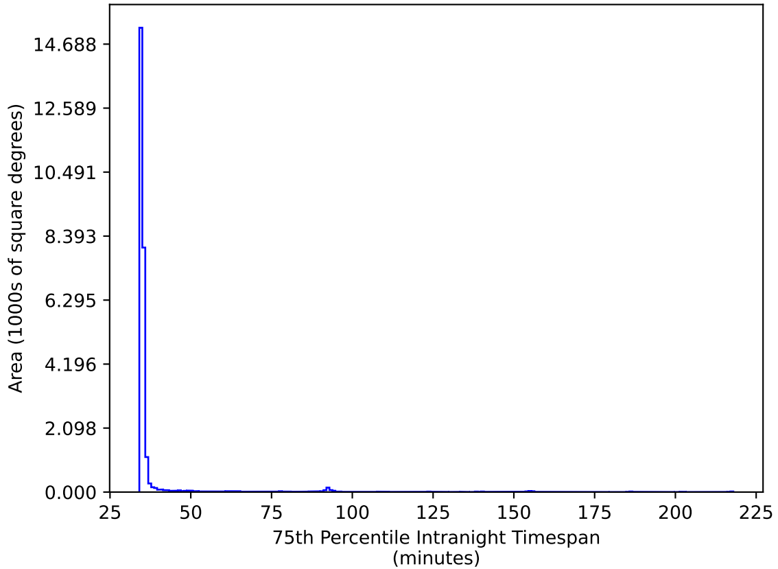
too_elab_heavy_r32_d2_griz_v3.4_10yrs All sky ri bands: 75th Percentile Intranight Timespan
