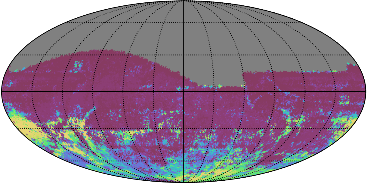
too_elab_heavy_r32_d2_griz_v3.4_10yrs All sky r band: 75th Percentile Intranight Timespan
