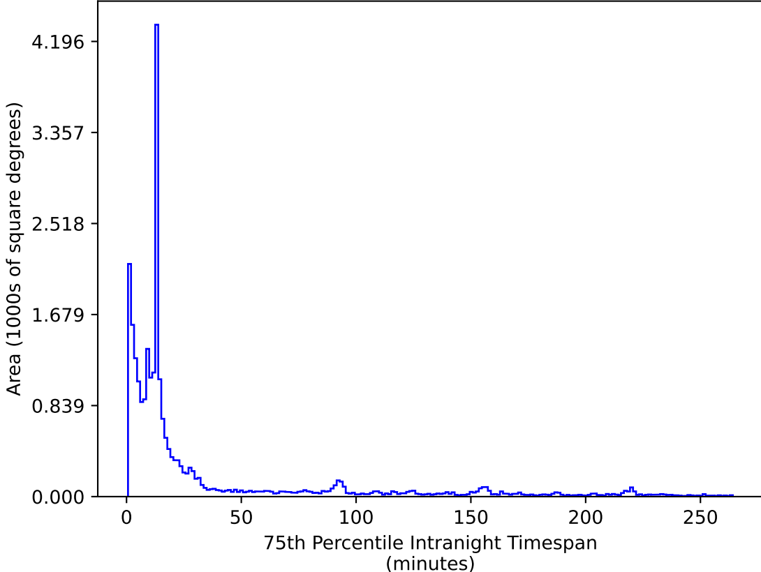
too_elab_heavy_r32_d2_griz_v3.4_10yrs All sky i band: 75th Percentile Intranight Timespan
