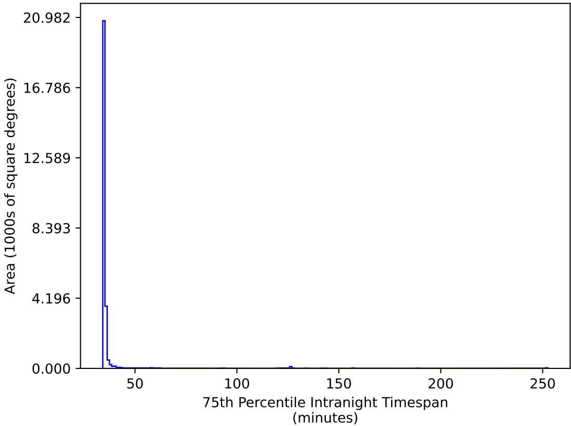
too_elab_heavy_r32_d2_griz_v3.4_10yrs All sky gr bands: 75th Percentile Intranight Timespan
