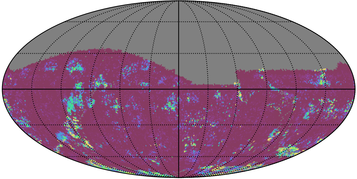
too_elab_heavy_r32_d2_griz_v3.4_10yrs All sky g band: 75th Percentile Intranight Timespan
