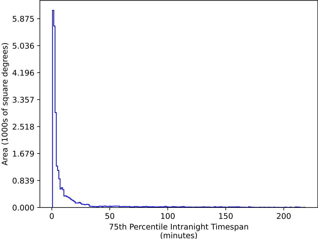
too_elab_heavy_r32_d2_griz_v3.4_10yrs All sky g band: 75th Percentile Intranight Timespan
