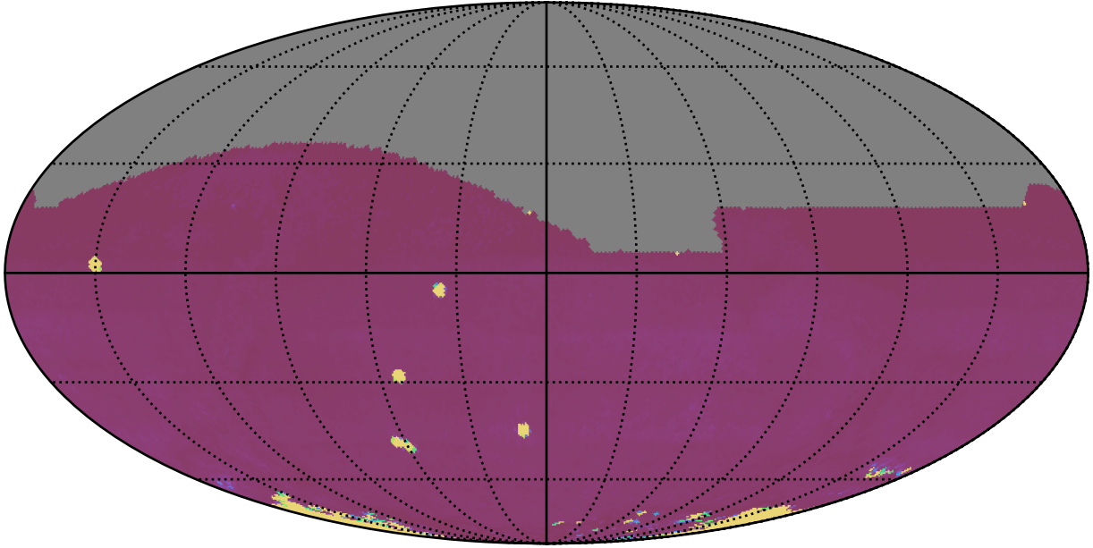
too_elab_heavy_r32_d2_griz_v3.4_10yrs All sky all bands: 75th Percentile Intranight Timespan
