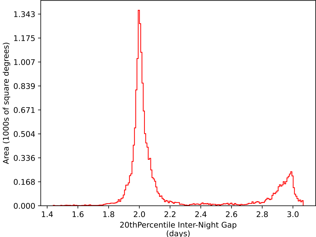
too_elab_heavy_r32_d2_griz_v3.4_10yrs WFD i band: 20thPercentile Inter-Night Gap
