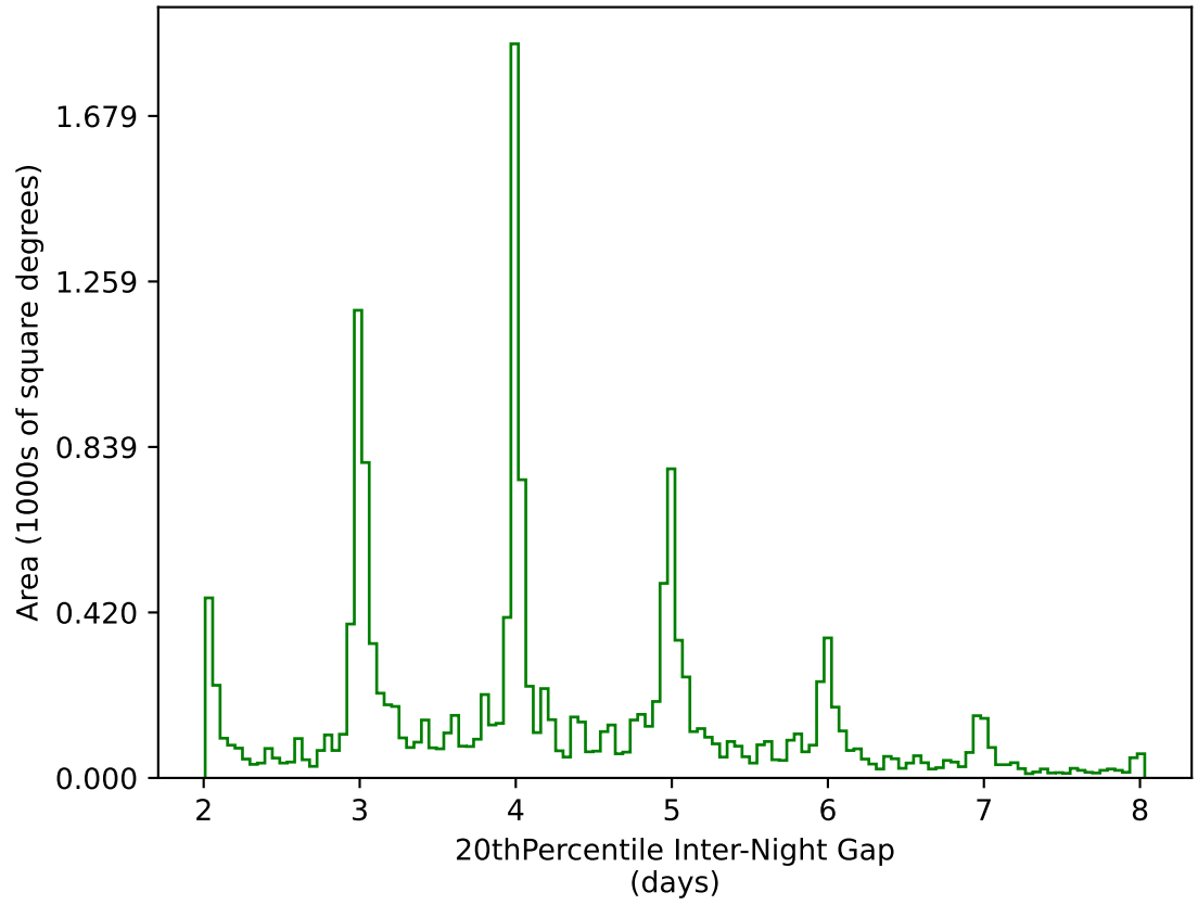
too_elab_heavy_r32_d2_griz_v3.4_10yrs WFD g band: 20thPercentile Inter-Night Gap
