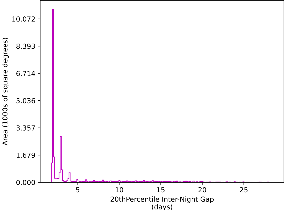
too_elab_heavy_r32_d2_griz_v3.4_10yrs All sky z band: 20thPercentile Inter-Night Gap
