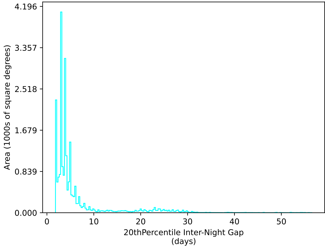
too_elab_heavy_r32_d2_griz_v3.4_10yrs All sky u band: 20thPercentile Inter-Night Gap
