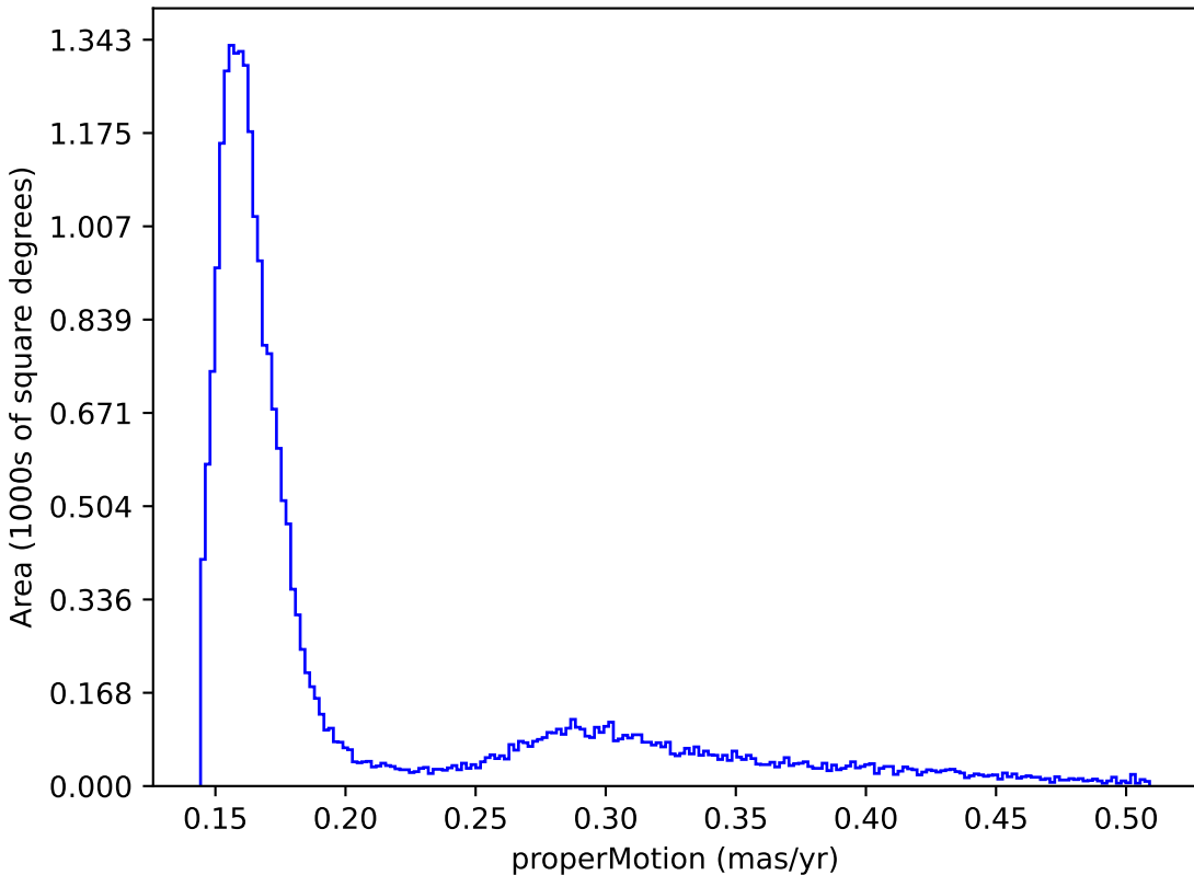
too_elab_heavy_r32_d2_griz_v3.4_10yrs : properMotion
