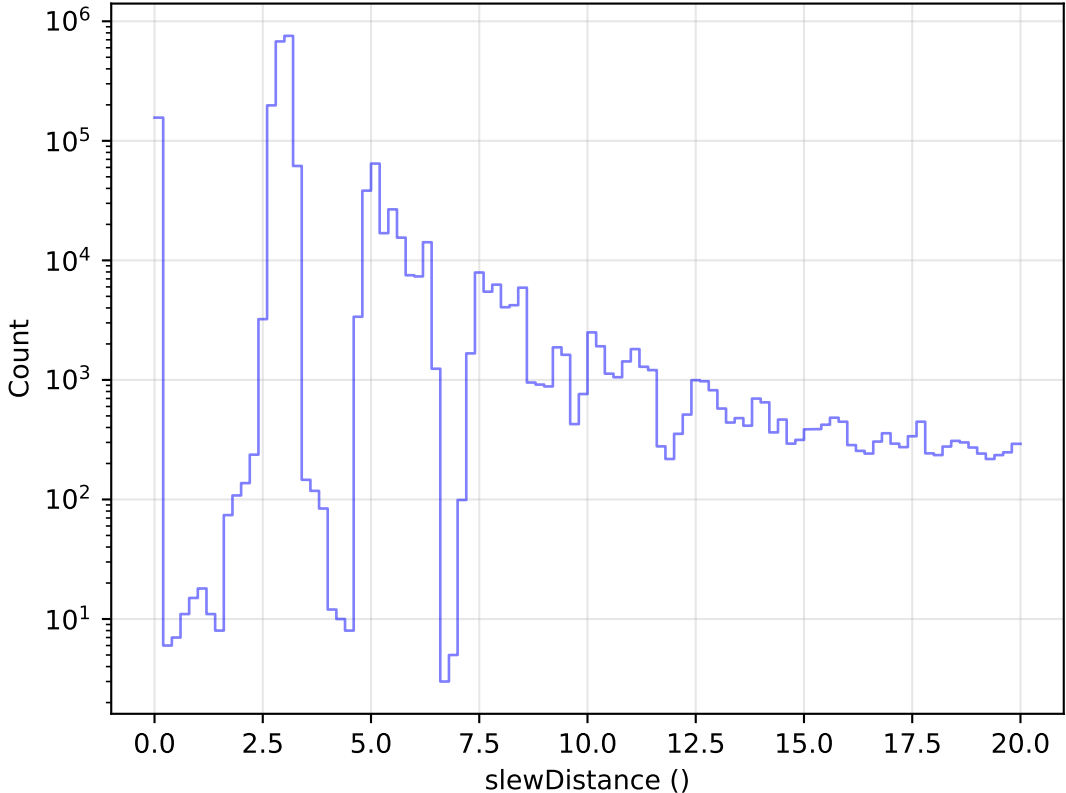
too_elab_heavy_r32_d2_griz_v3.4_10yrs All visits: Zoom Slew Distance Histogram
