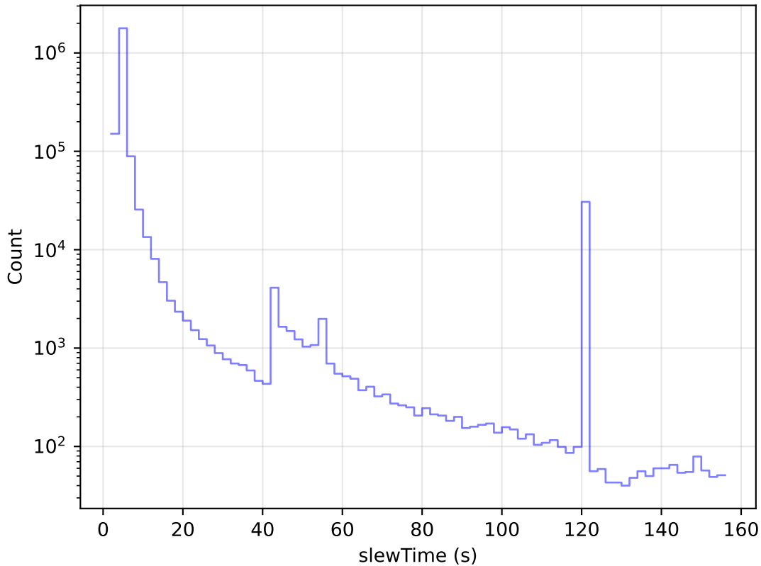
too_elab_heavy_r32_d2_griz_v3.4_10yrs All visits: Slew Time Histogram
