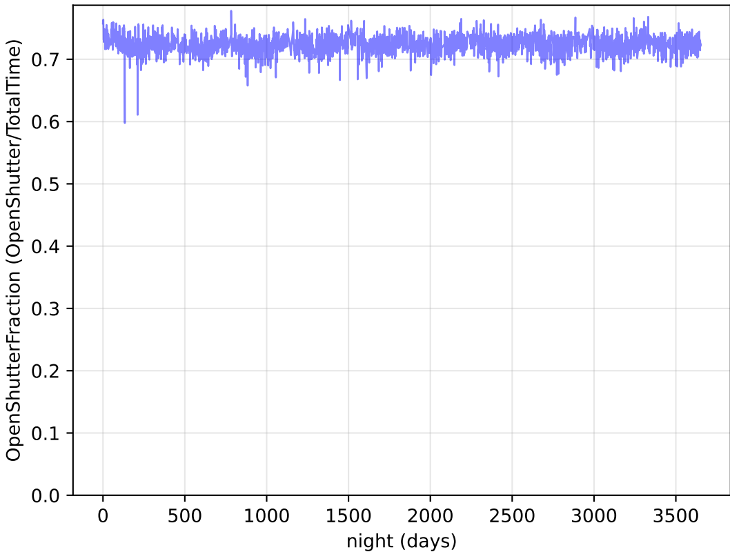
too_elab_heavy_r32_d2_griz_v3.4_10yrs : OpenShutterFraction
