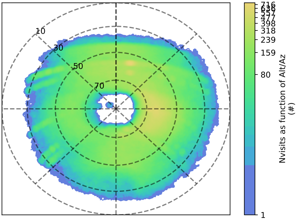
too_elab_heavy_r32_d2_griz_v3.4_10yrs u: Nvisits as function of Alt/Az
