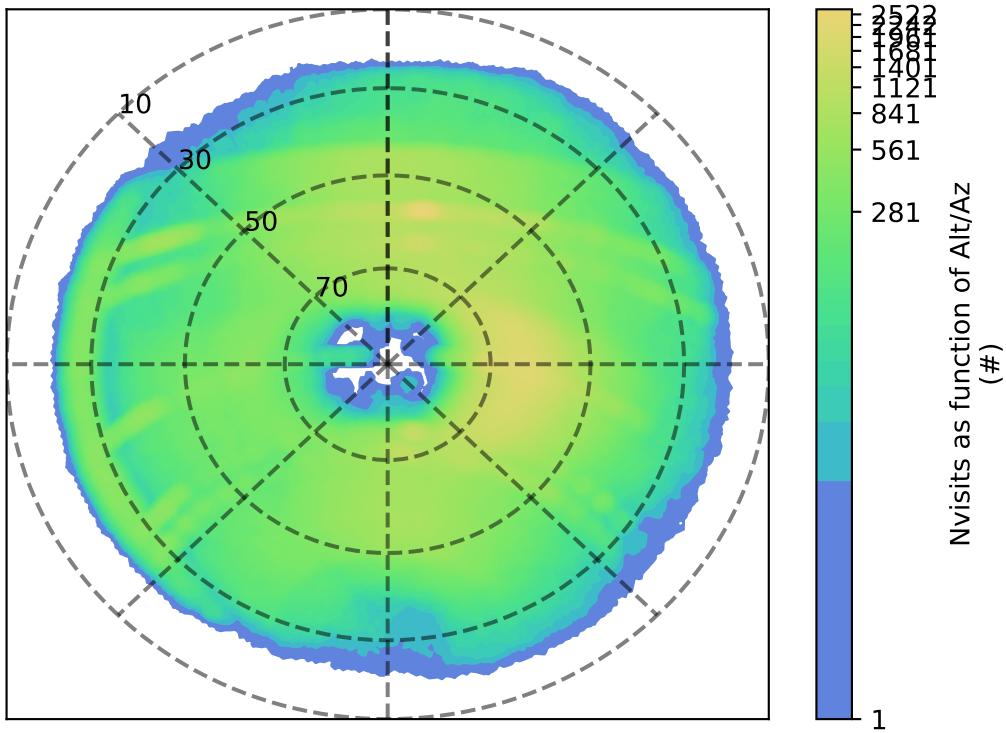
too_elab_heavy_r32_d2_griz_v3.4_10yrs r: Nvisits as function of Alt/Az
