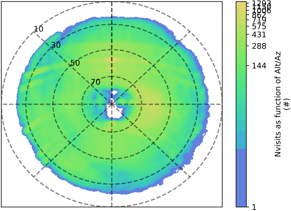
too_elab_heavy_r32_d2_griz_v3.4_10yrs g: Nvisits as function of Alt/Az
