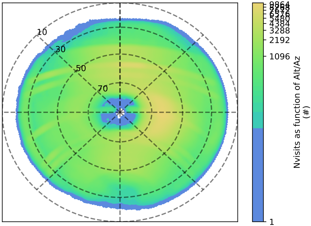
too_elab_heavy_r32_d2_griz_v3.4_10yrs : Nvisits as function of Alt/Az
