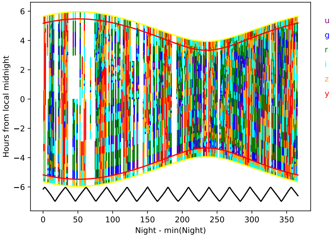
too_elab_heavy_r32_d2_griz_v3.4_10yrs year 9-10: Hourglass
