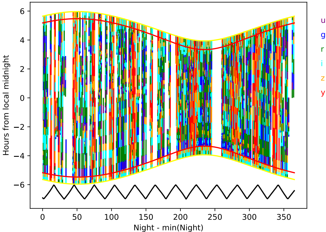
too_elab_heavy_r32_d2_griz_v3.4_10yrs year 5-6: Hourglass
