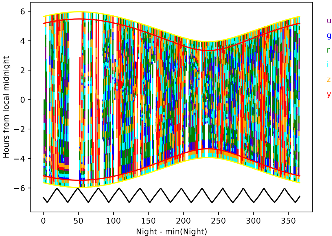
too_elab_heavy_r32_d2_griz_v3.4_10yrs year 2-3: Hourglass
