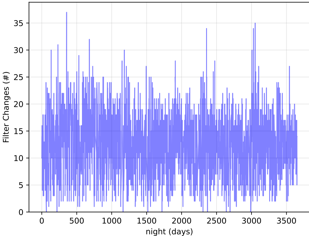
too_elab_heavy_r32_d2_griz_v3.4_10yrs : Filter Changes
