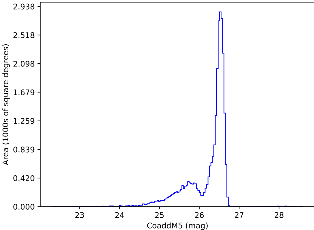
too_elab_heavy_r32_d2_griz_v3.4_10yrs i: CoaddM5
