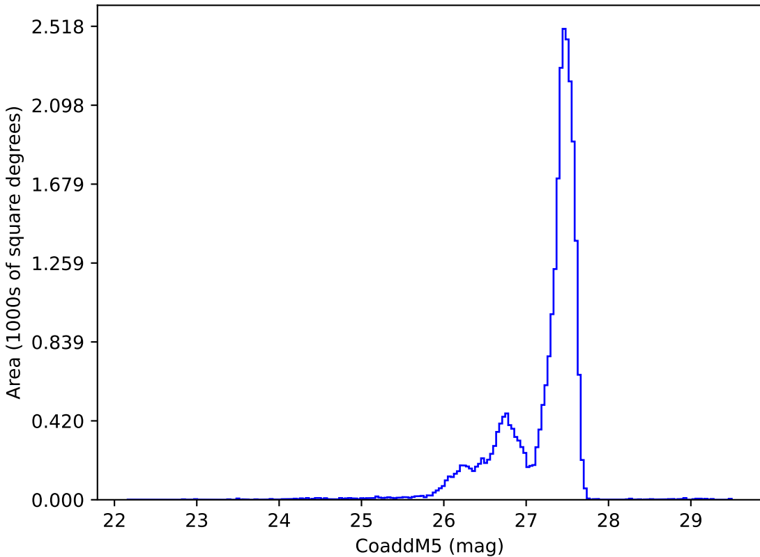
too_elab_heavy_r32_d2_griz_v3.4_10yrs : CoaddM5
