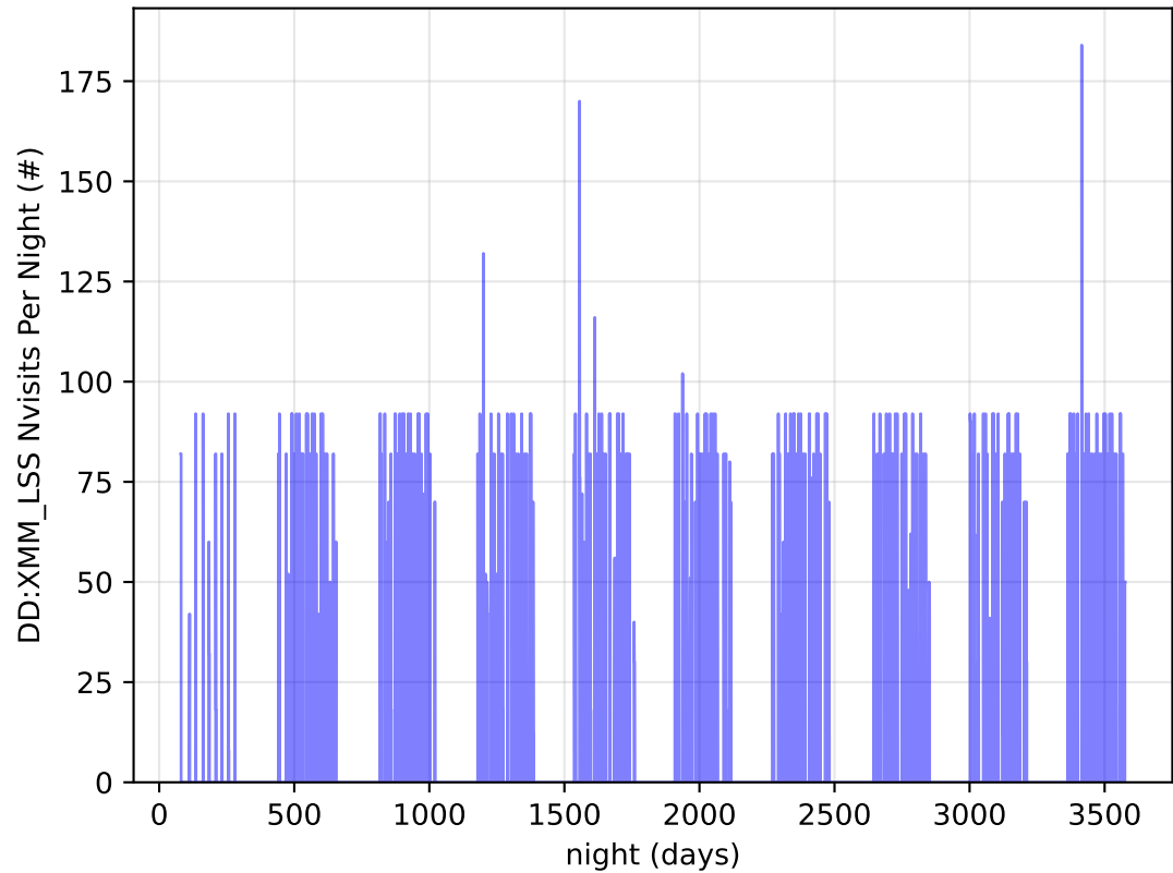
too_elab_heavy_r32_d2_griz_v3.4_10yrs all bands: DD:XMM_LSS Nvisits Per Night
