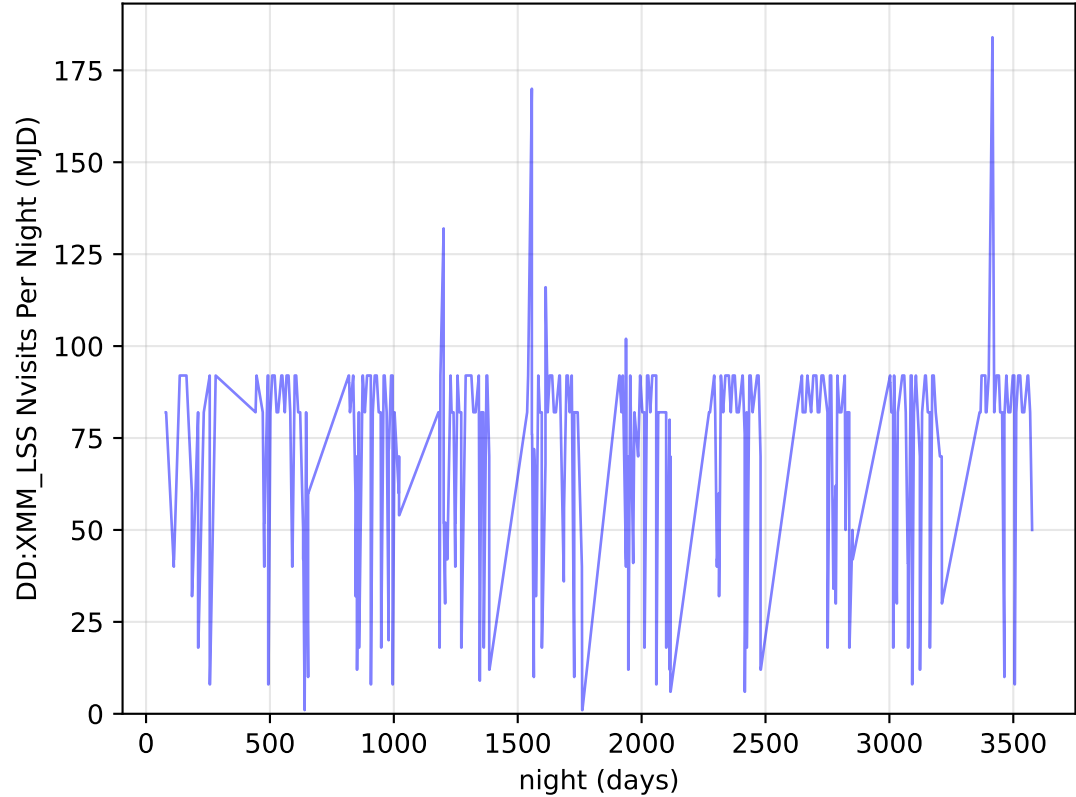
too_elab_heavy_r32_d2_griz_v3.4_10yrs all bands: DD:XMM_LSS Nvisits Per Night
