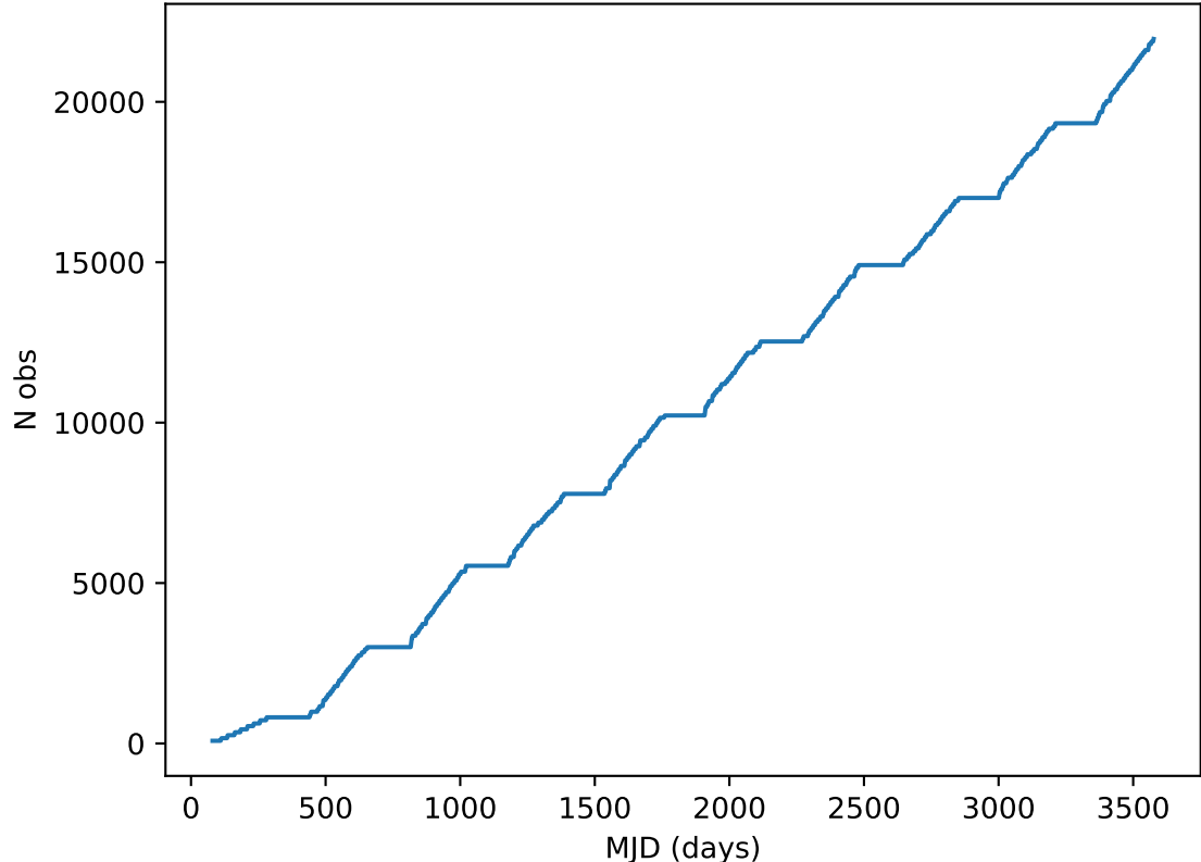
too_elab_heavy_r32_d2_griz_v3.4_10yrs all bands: DD:XMM_LSS Cumulative NVisits
