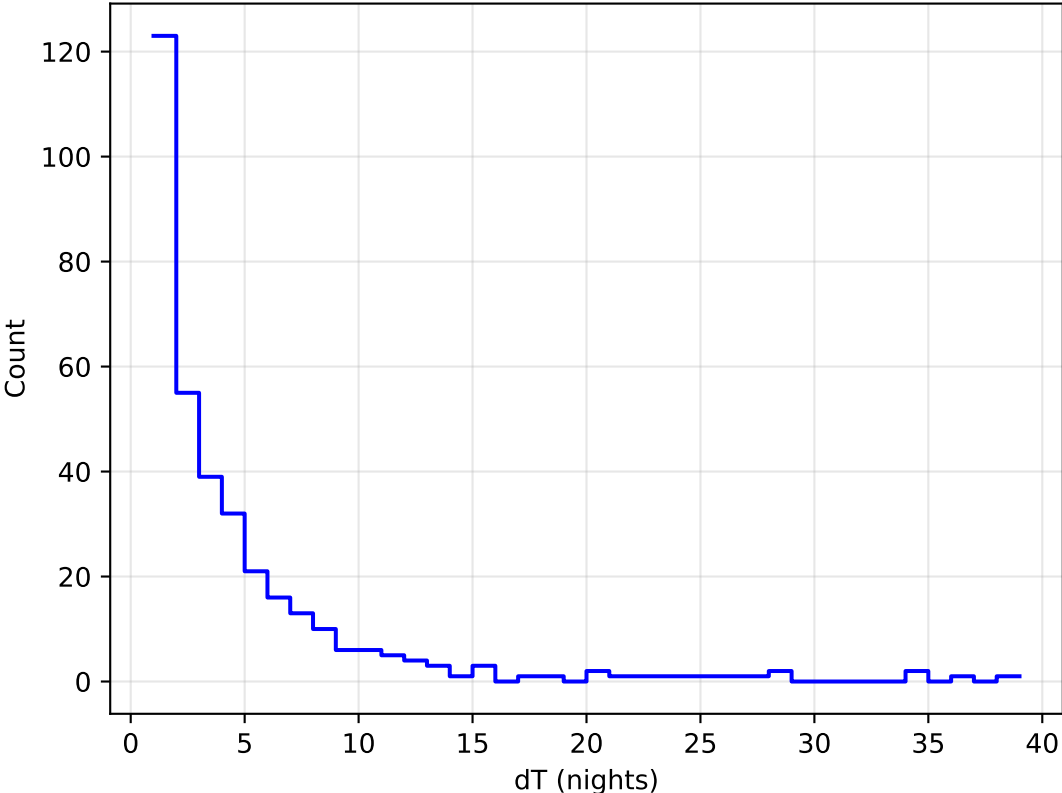
too_elab_heavy_r32_d2_griz_v3.4_10yrs all bands: DD:WFD Delta Nights Histogram
