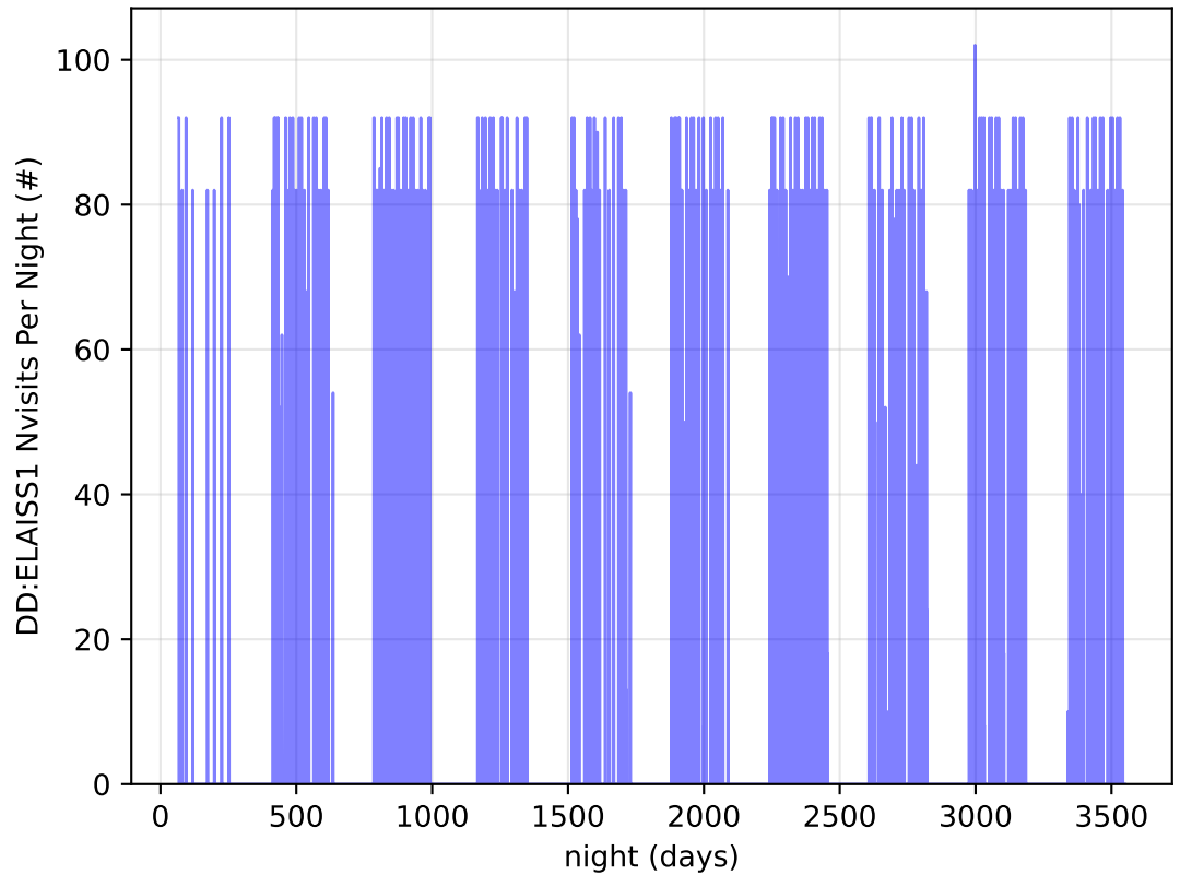
too_elab_heavy_r32_d2_griz_v3.4_10yrs all bands: DD:ELAISS1 Nvisits Per Night
