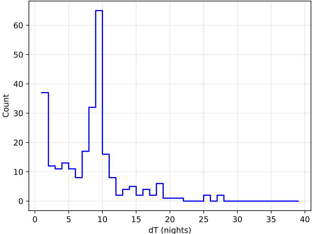
too_elab_heavy_r32_d2_griz_v3.4_10yrs all bands: DD:ELAISS1 Delta Nights Histogram
