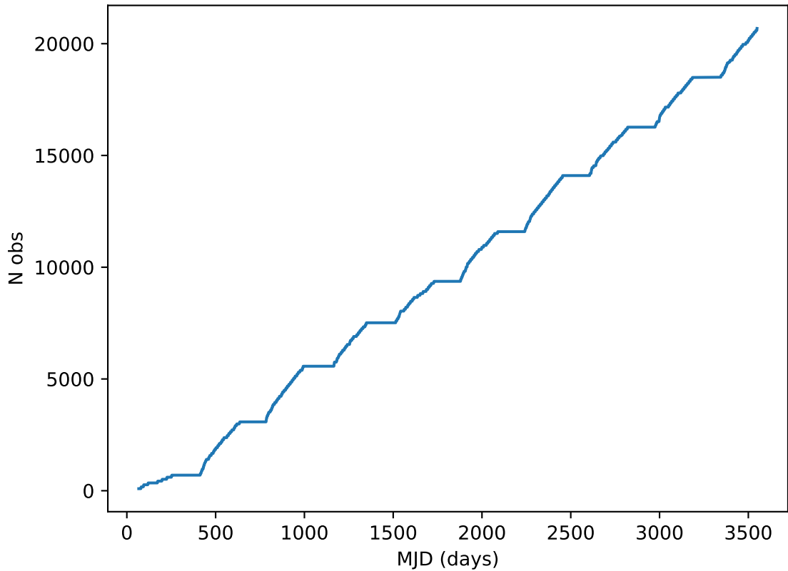
too_elab_heavy_r32_d2_griz_v3.4_10yrs all bands: DD:ELAISS1 Cumulative NVisits
