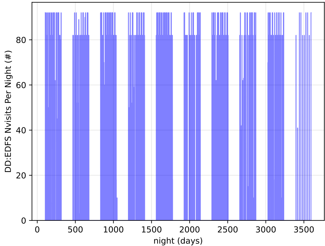
too_elab_heavy_r32_d2_griz_v3.4_10yrs all bands: DD:EDFS Nvisits Per Night
