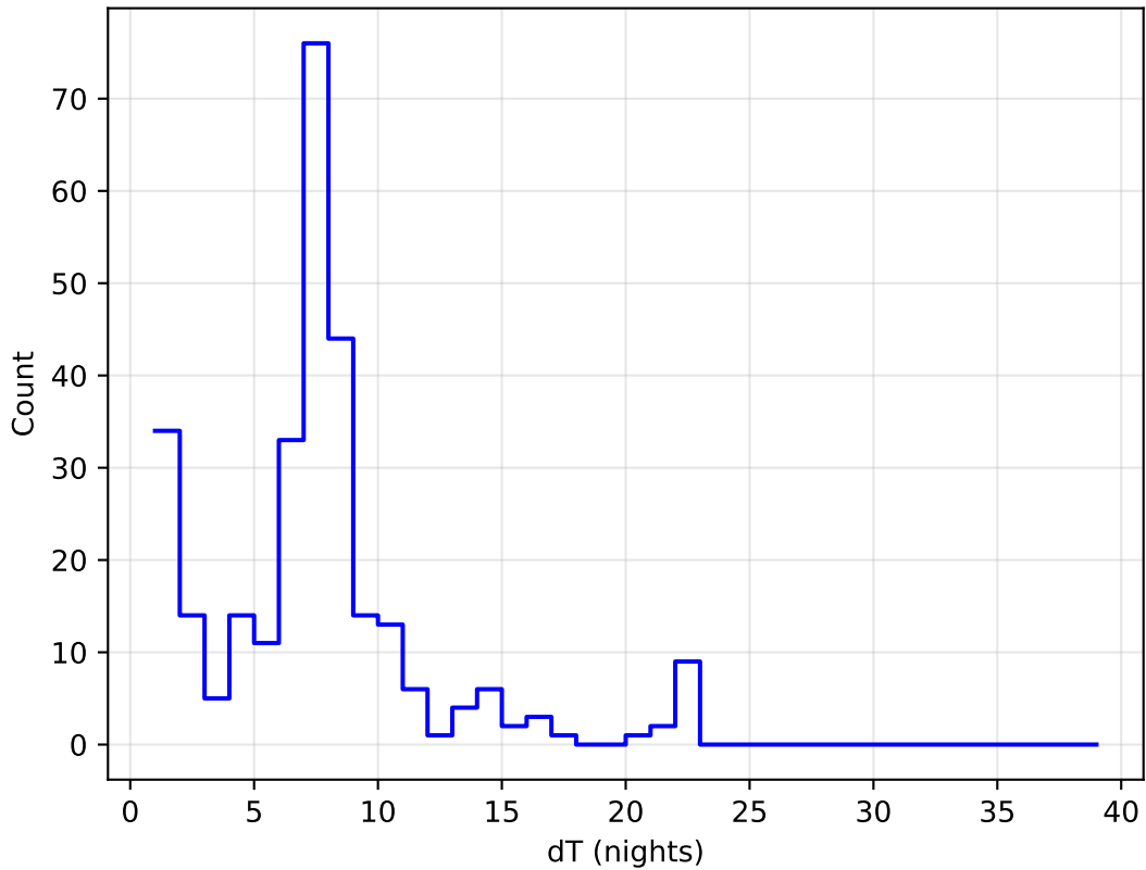
too_elab_heavy_r32_d2_griz_v3.4_10yrs all bands: DD:EDFS Delta Nights Histogram
