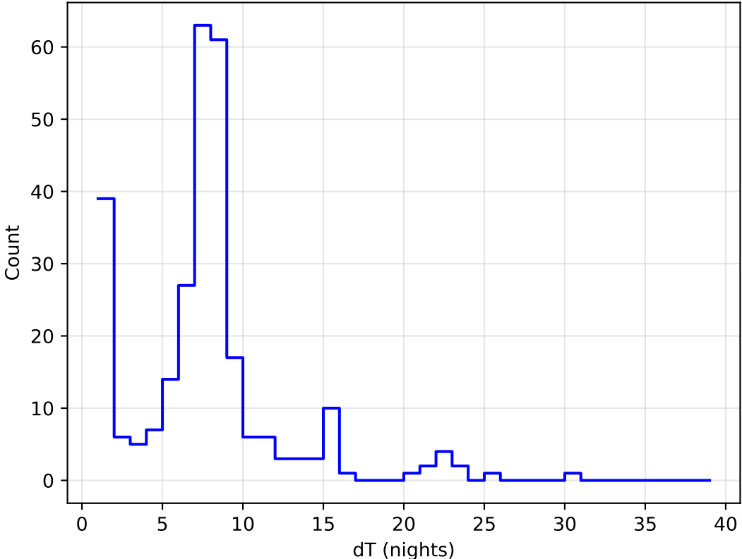
too_elab_heavy_r32_d2_griz_v3.4_10yrs all bands: DD:ECDFS Delta Nights Histogram
