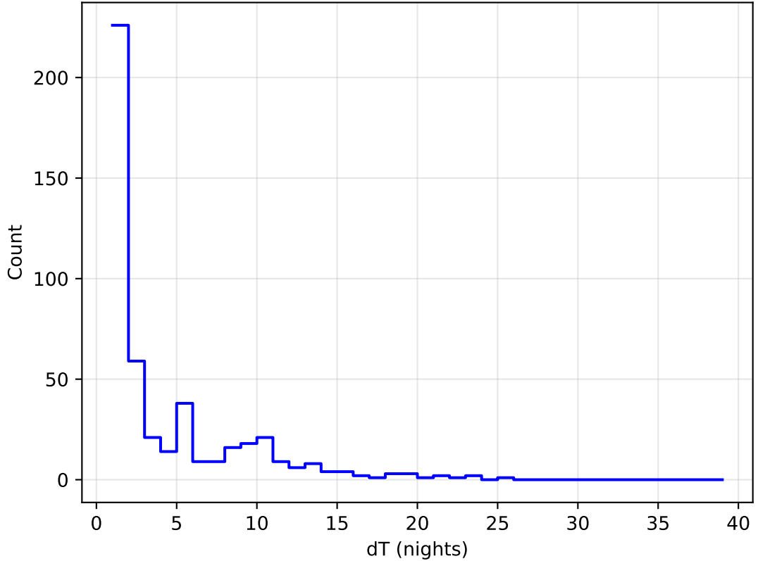
too_elab_heavy_r32_d2_griz_v3.4_10yrs all bands: DD: COSMOS Delta Nights Histogram
