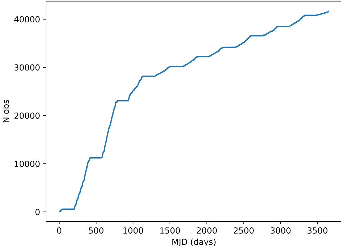
too_elab_heavy_r32_d2_griz_v3.4_10yrs all bands: DD:COSMOS Cumulative NVisits
