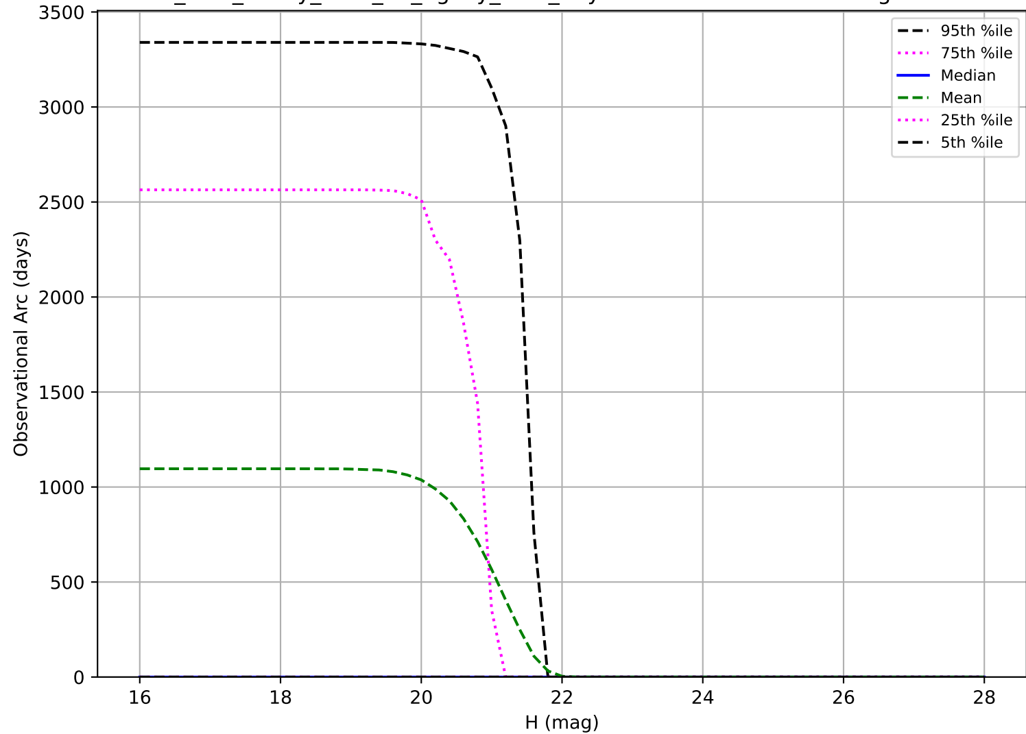
too_elab_heavy_r128_d3_ugrizy_v3.4_10yrs: Observational Arc Length Vatira
