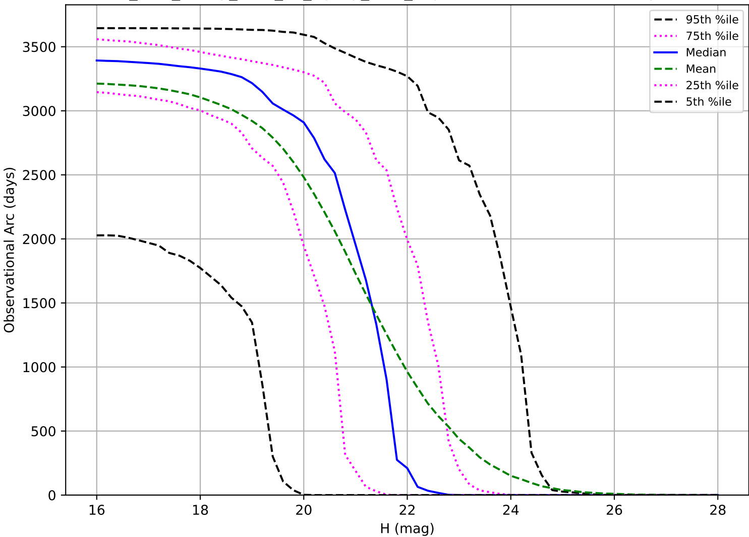
too_elab_heavy_r128_d3_ugrizy_v3.4_10yrs: Observational Arc Length PHA
