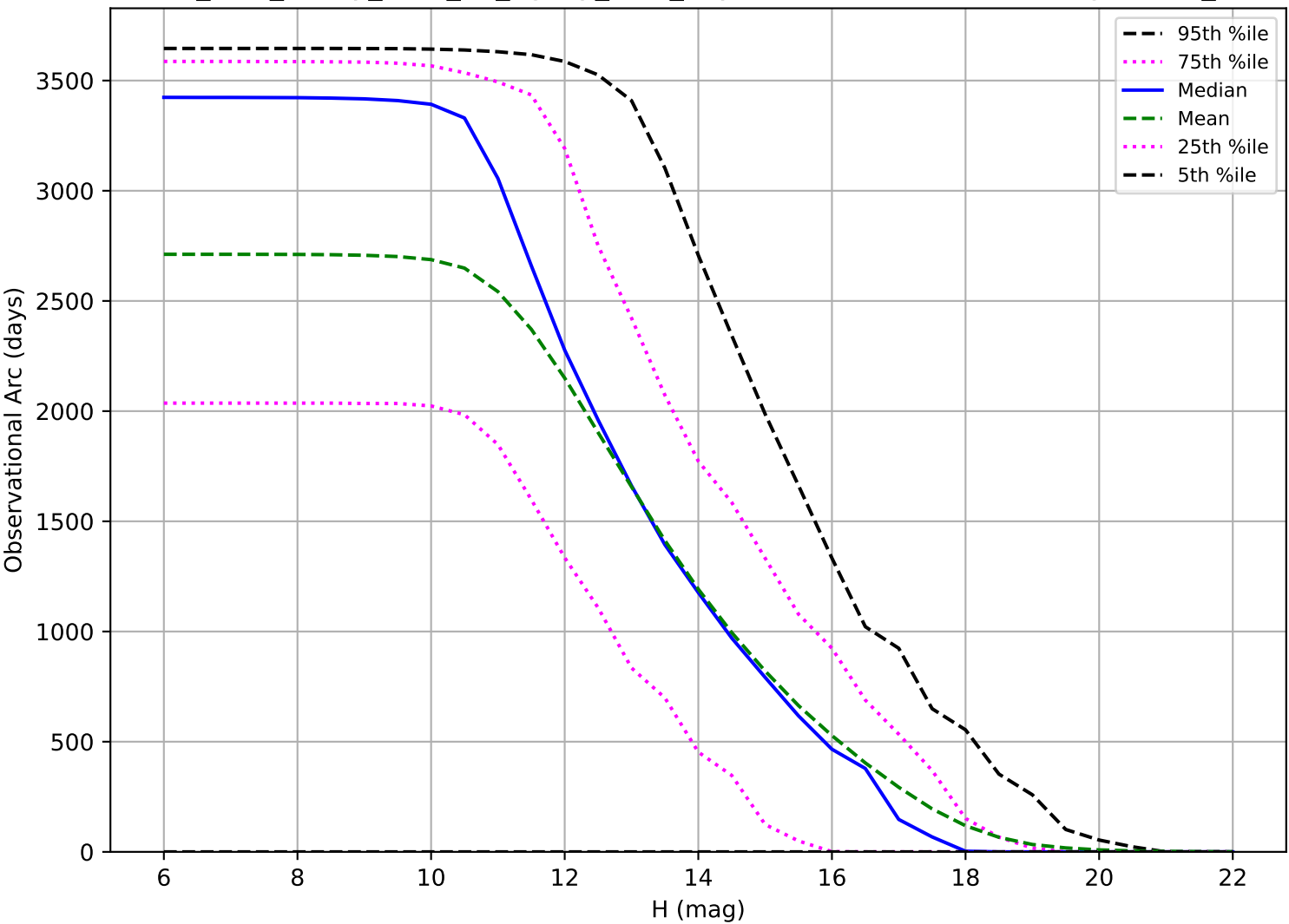
too_elab_heavy_r128_d3_ugrizy_v3.4_10yrs: Observational Arc Length OCC_r5
