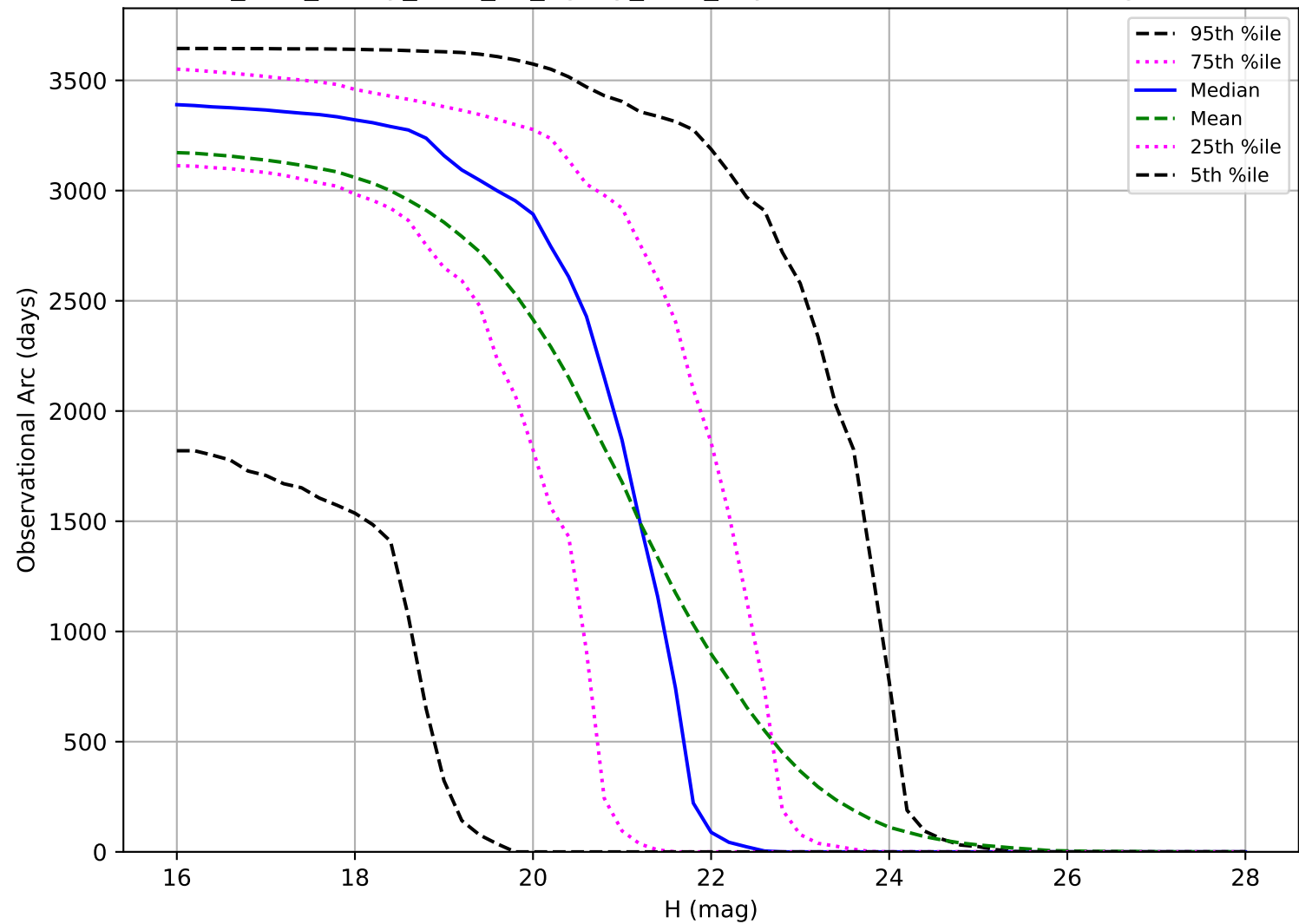
too_elab_heavy_r128_d3_ugrizy_v3.4_10yrs: Observational Arc Length NEO
