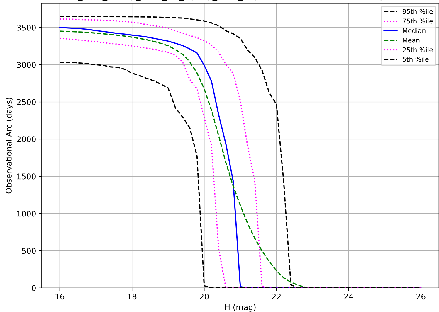
too_elab_heavy_r128_d3_ugrizy_v3.4_10yrs: Observational Arc Length MBA
