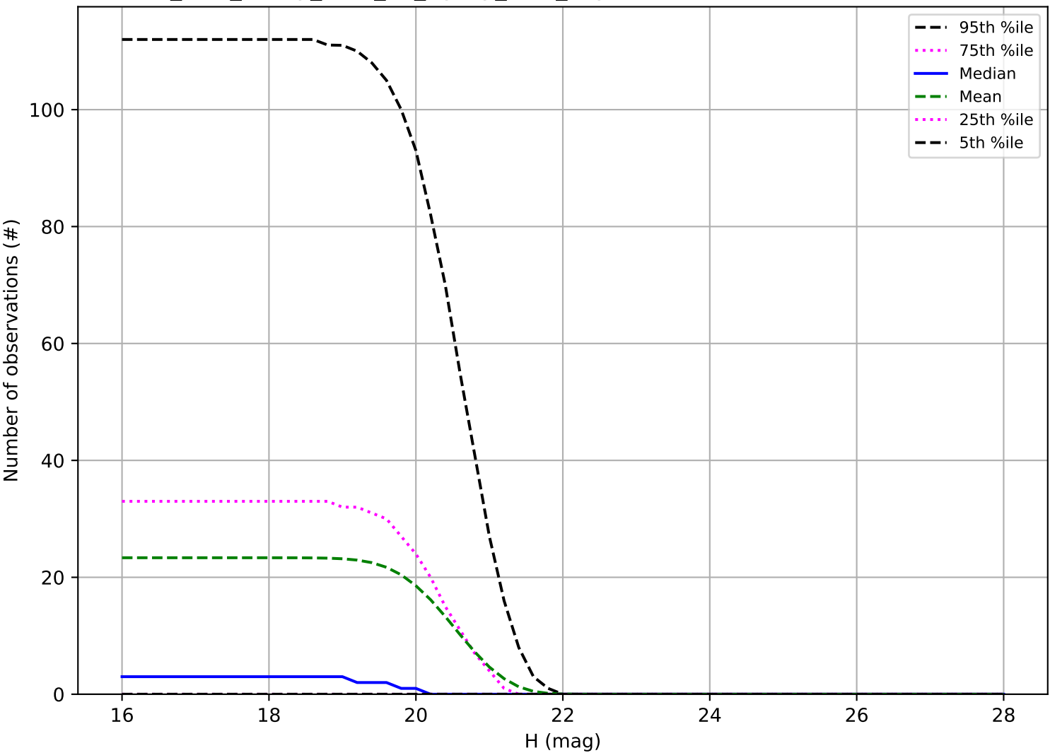
too_elab_heavy_r128_d3_ugrizy_v3.4_10yrs: Number of observations Vatira
