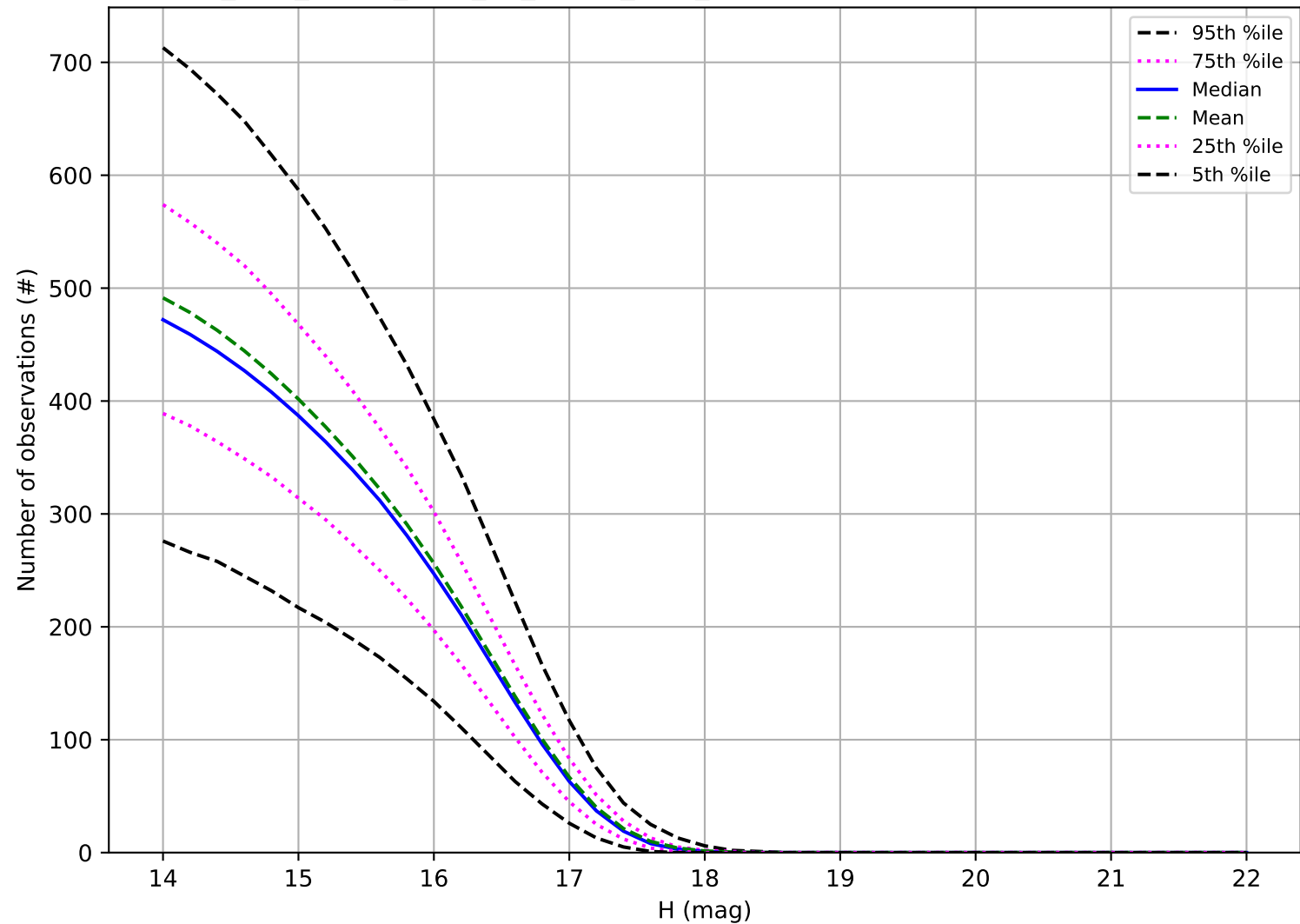
too_elab_heavy_r128_d3_ugrizy_v3.4_10yrs: Number of observations Trojan
