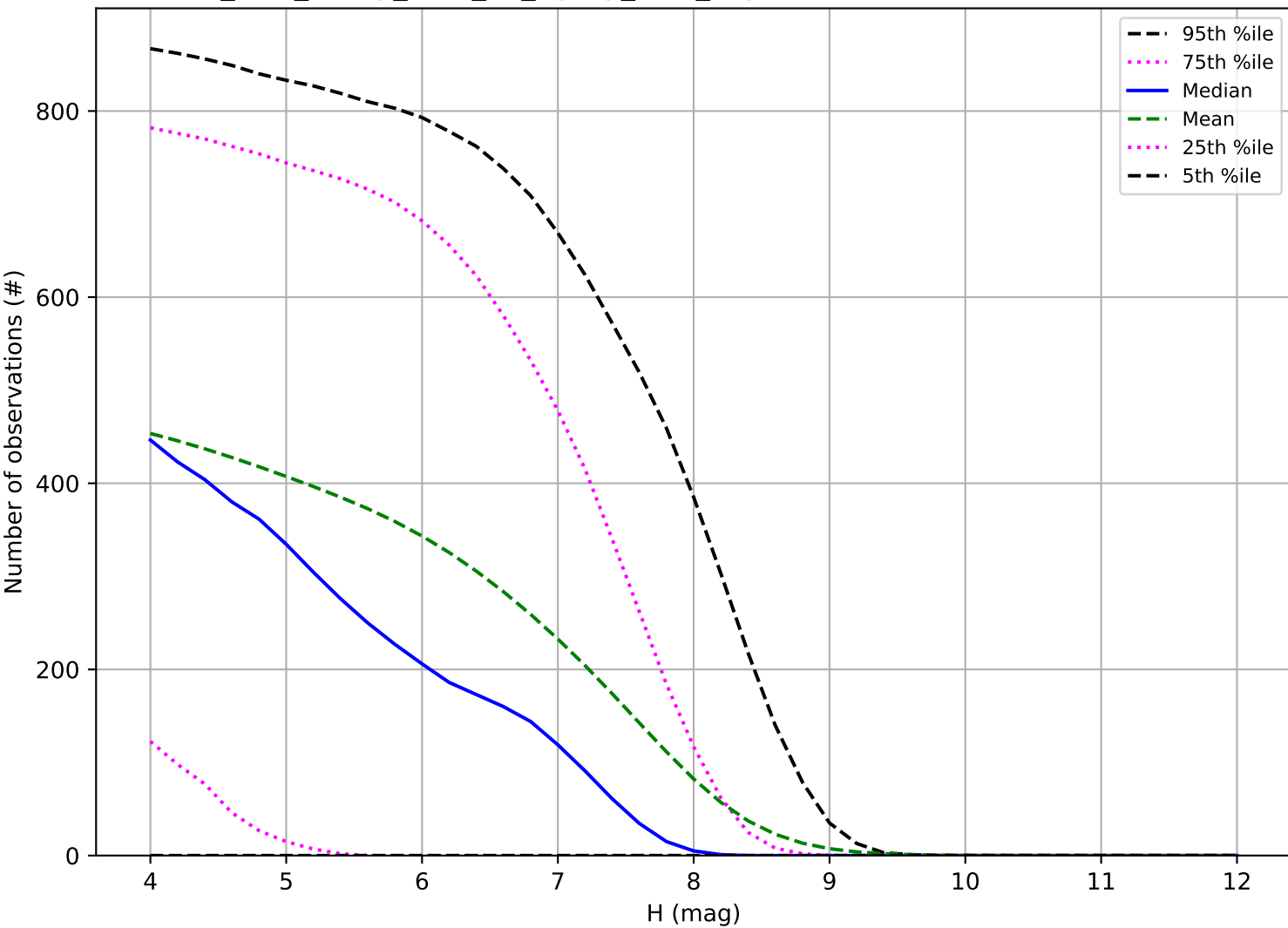
too_elab_heavy_r128_d3_ugrizy_v3.4_10yrs: Number of observations TNO
