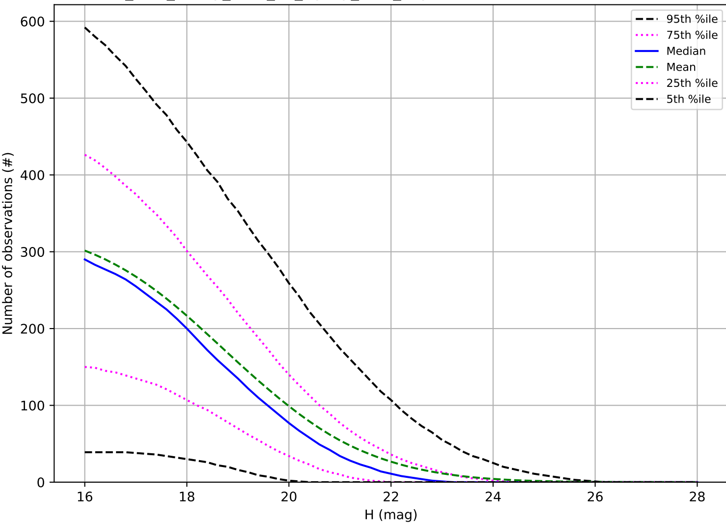
too_elab_heavy_r128_d3_ugrizy_v3.4_10yrs: Number of observations PHA
