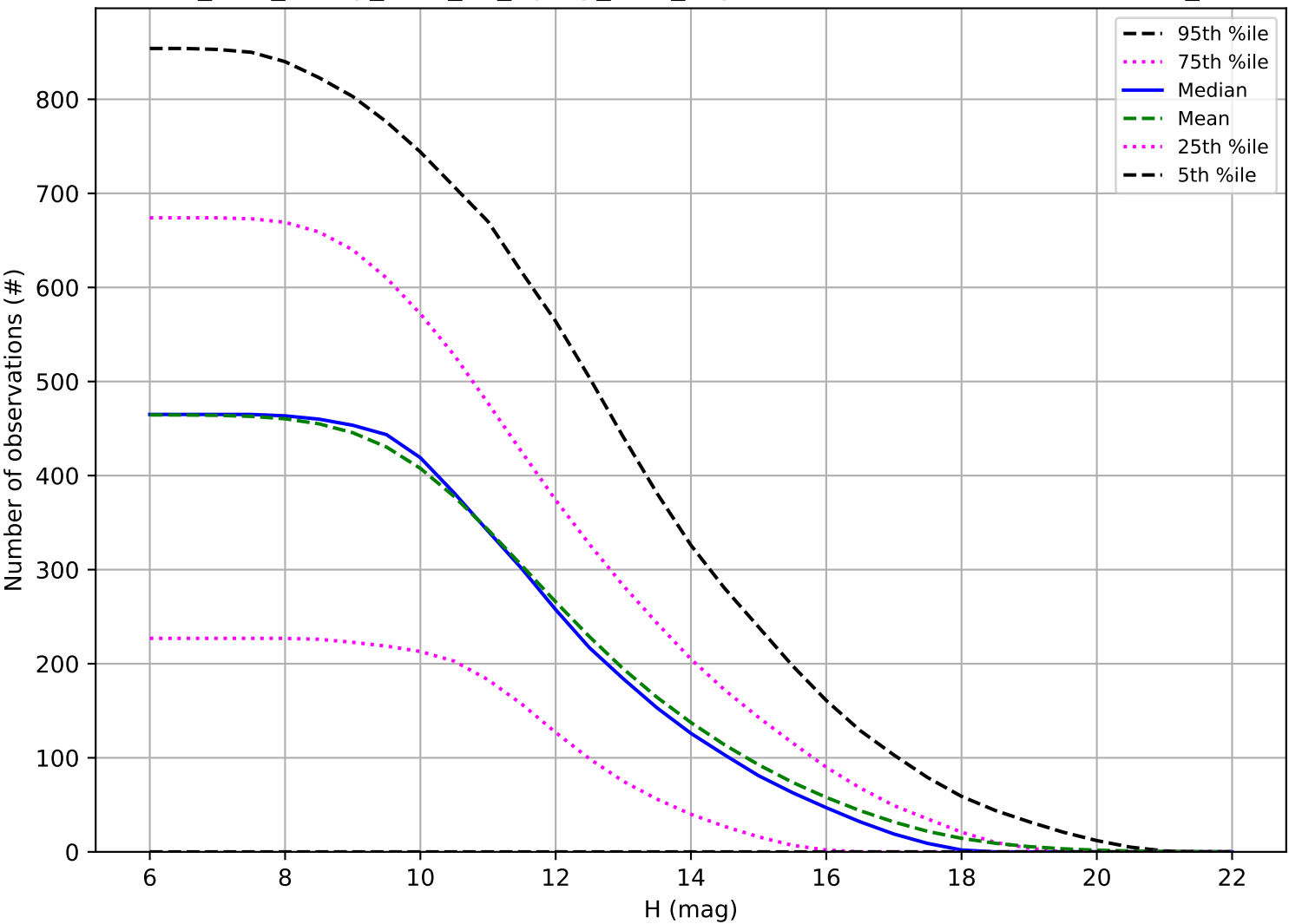
too_elab_heavy_r128_d3_ugrizy_v3.4_10yrs: Number of observations OCC_r5
