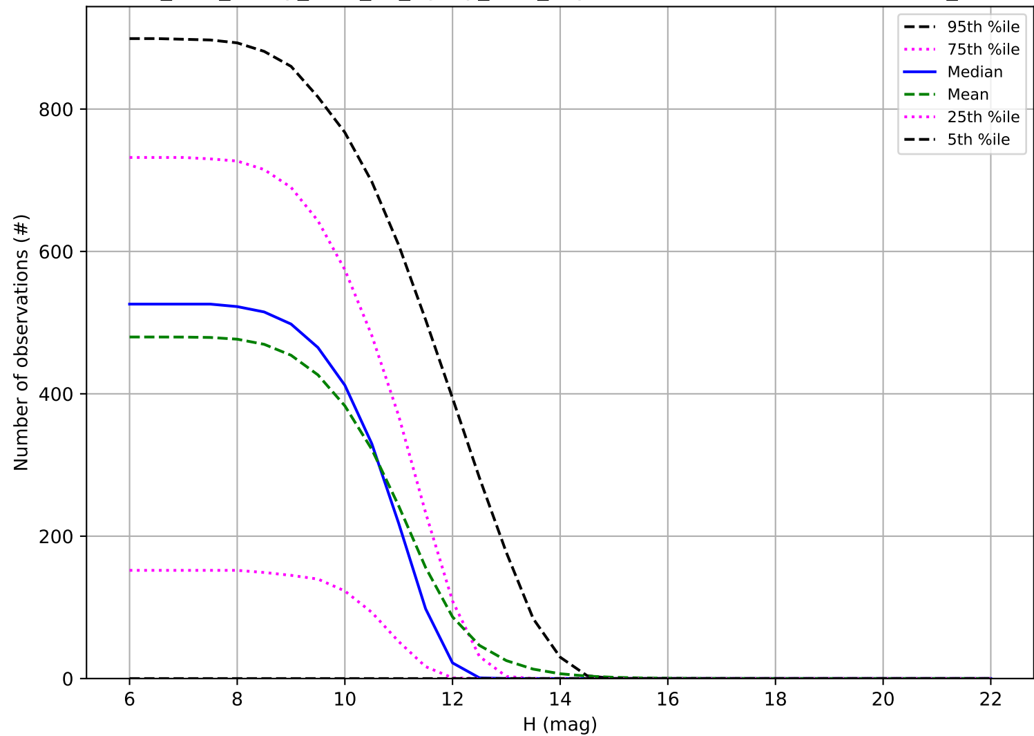
too_elab_heavy_r128_d3_ugrizy_v3.4_10yrs: Number of observations OCC_r20
