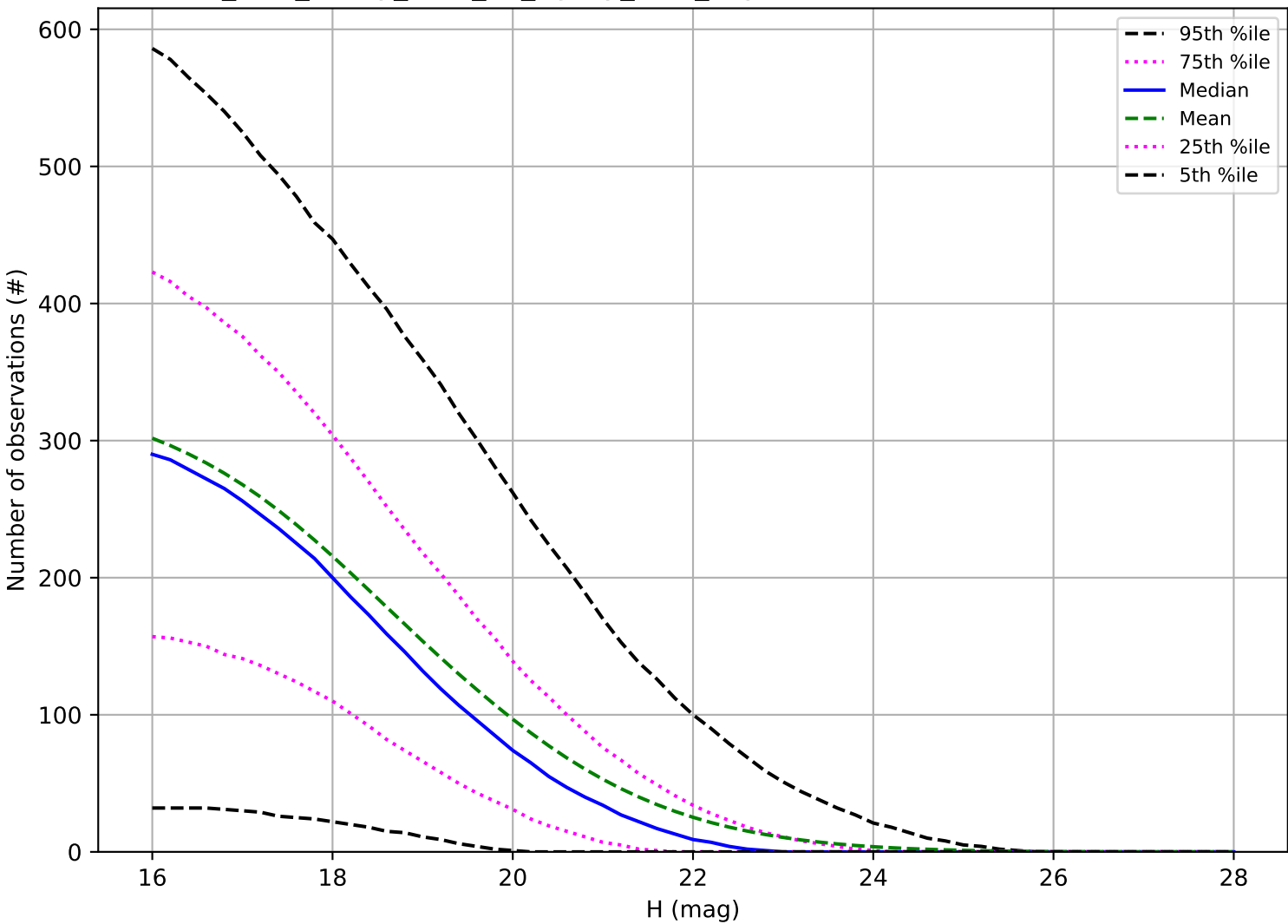
too_elab_heavy_r128_d3_ugrizy_v3.4_10yrs: Number of observations NEO
