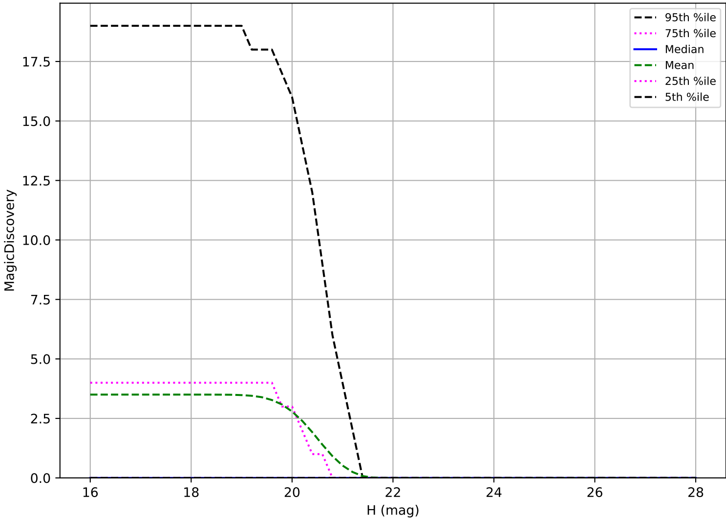
too_elab_heavy_r128_d3_ugrizy_v3.4_10yrs: Vatira 6 detections in 60 nights detection loss
